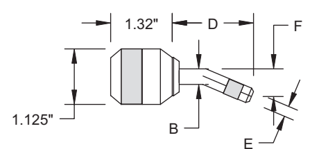
CURVED NOSE
